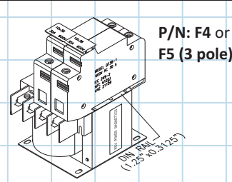
Fig. 3 - Rejection type, CE marked touch safe, 600 V max, din rail mtg.
