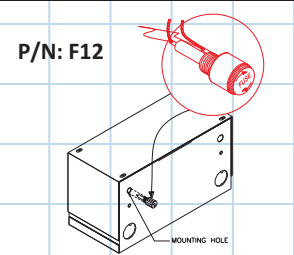
Fig. 4 - For enclosed units. 250 V max c/w pigtails, Fuse size: 1/4 x 1/4
