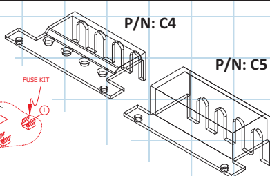
Fig. 2 - Touch Safe Terminal Covers
