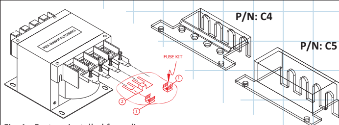
Fig. 1 - Factory installed fuse clip Secondary side (250 V max) Fuse size: 13/32 x 1 1/2
