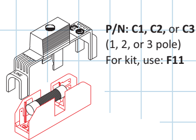
Fig. 6 - Touch-safe cover for non-rejection type
